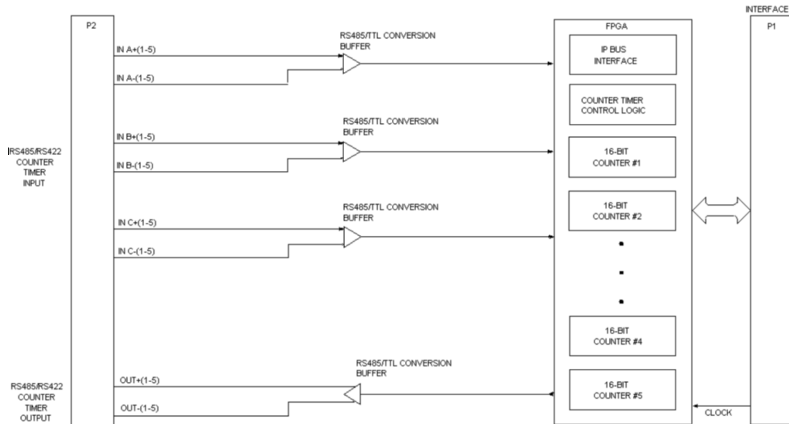
IP484 BLOCK DIAGRAM
