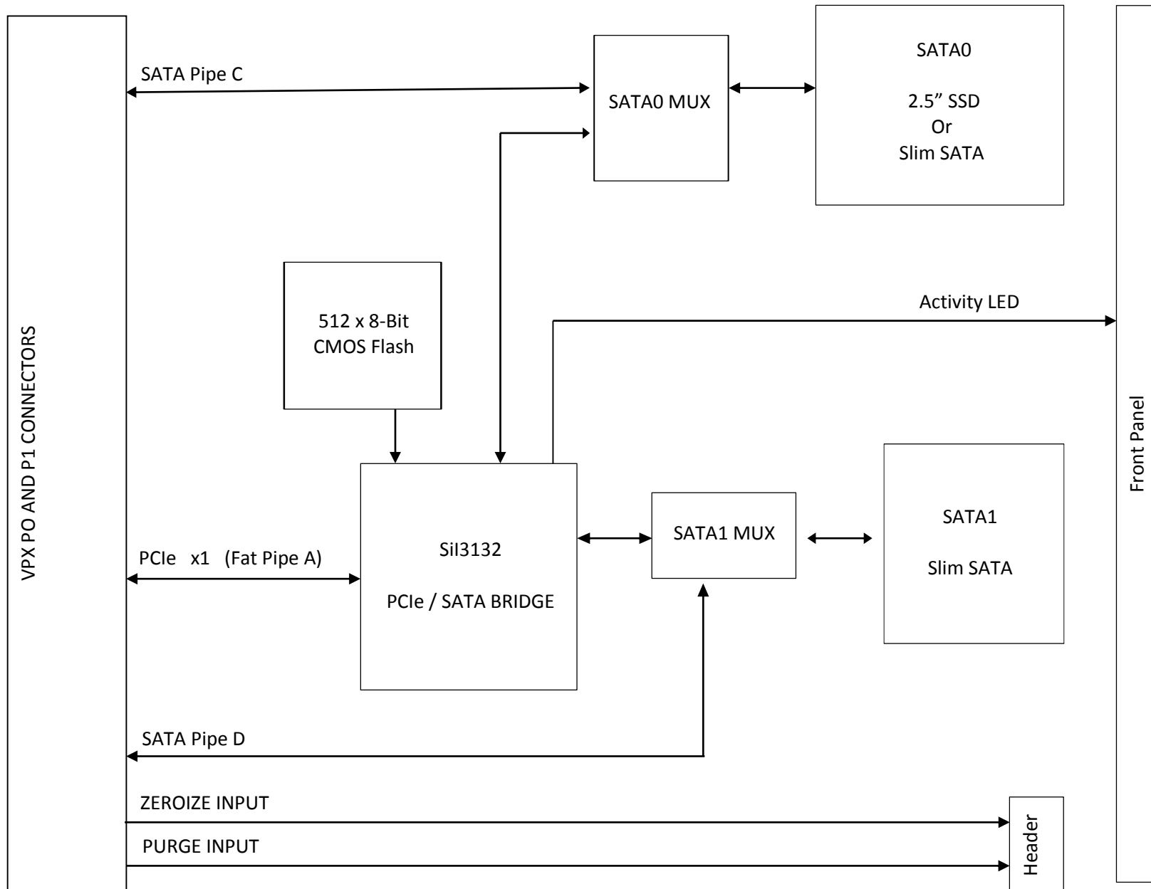
XVPX-9756 Block Diagram
