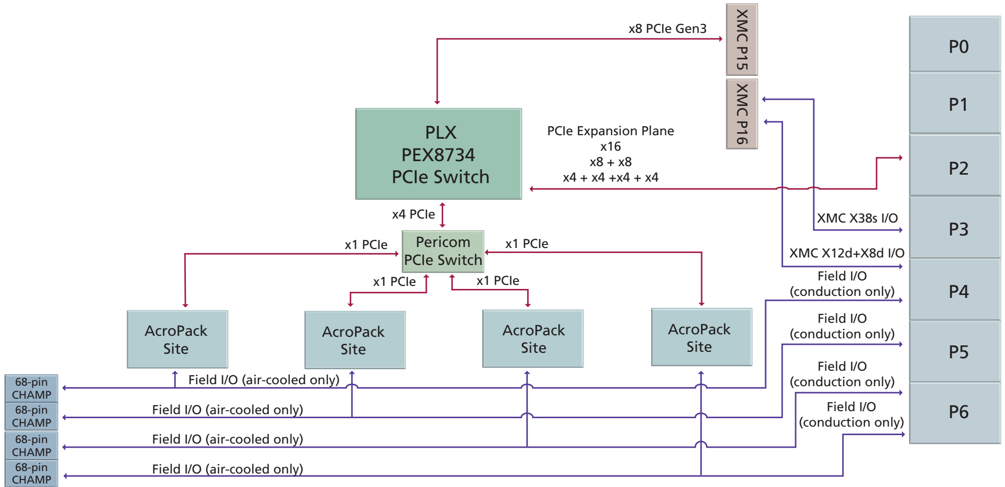
VPX4520 Block Diagram
