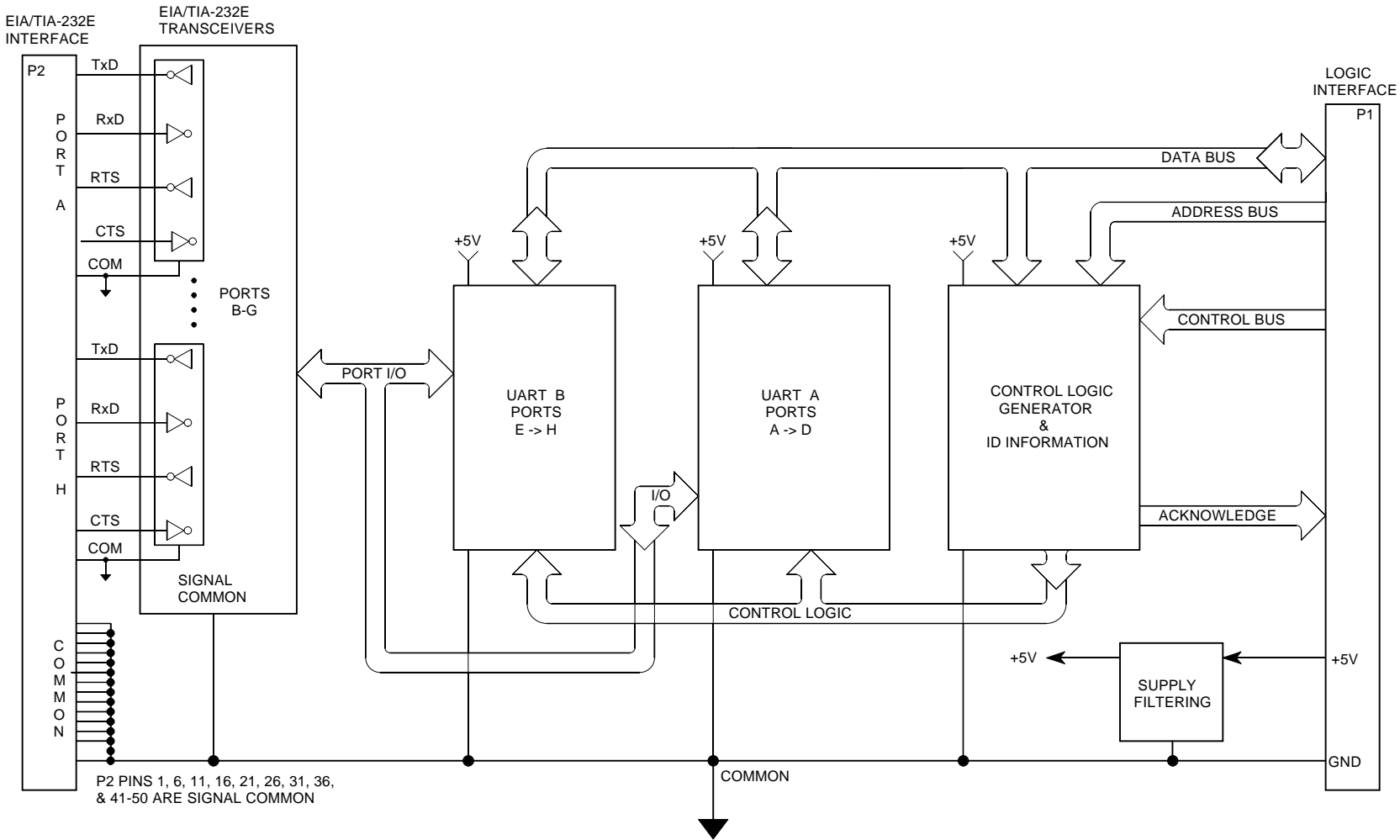
IP520 BLOCK DIAGRAM
