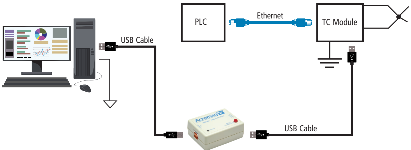
Figure 3: Differing grounds is another situation where USB isolation should be used.
