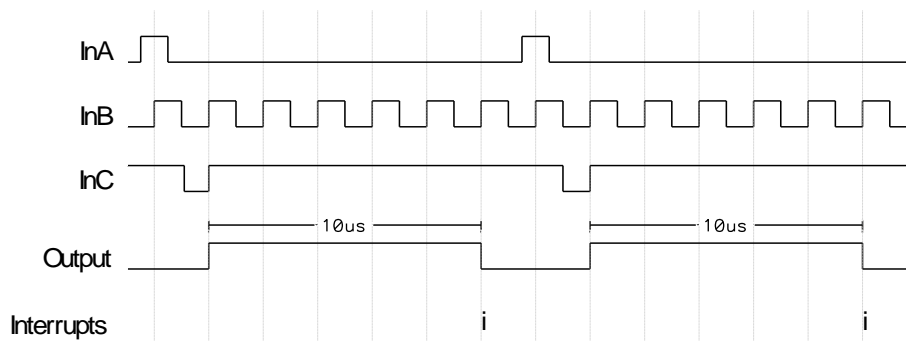
Figure 3.4: Watchdog waveform
