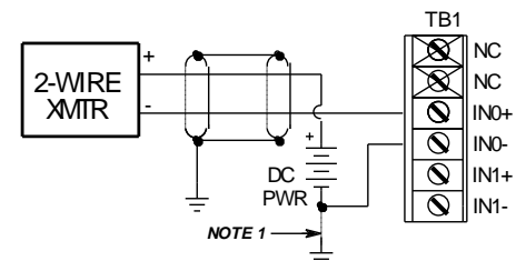
2-WIRE TRANSMITTER (961EN)
