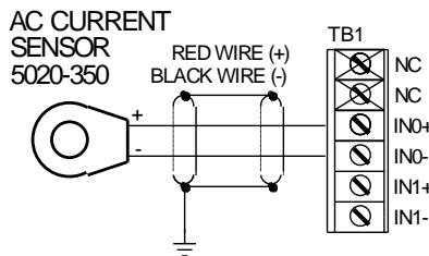
AC CURRENT SENSOR INPUT (961EN)
