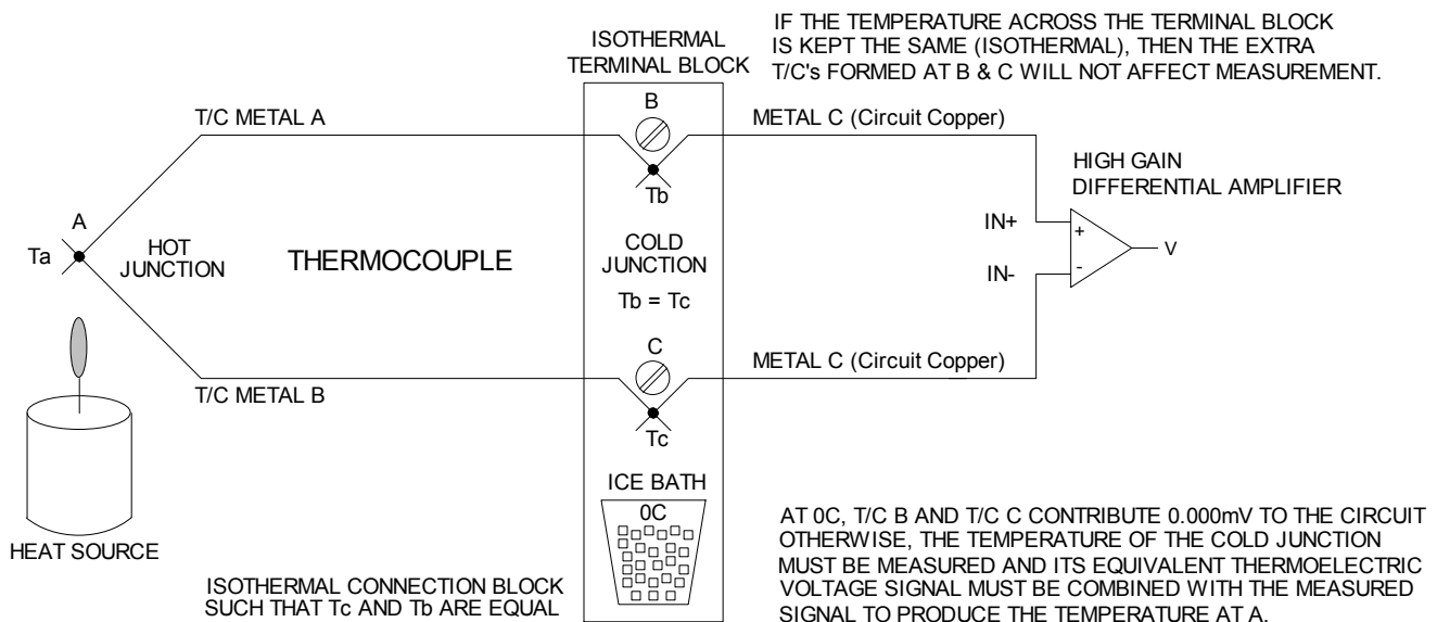
FIGURE 1: A SIMPLIFIED THERMOCOUPLE MEASURING CIRCUIT
